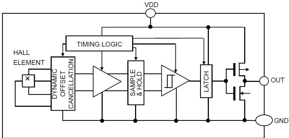
Figure 2, Block Diagram of AS1832
