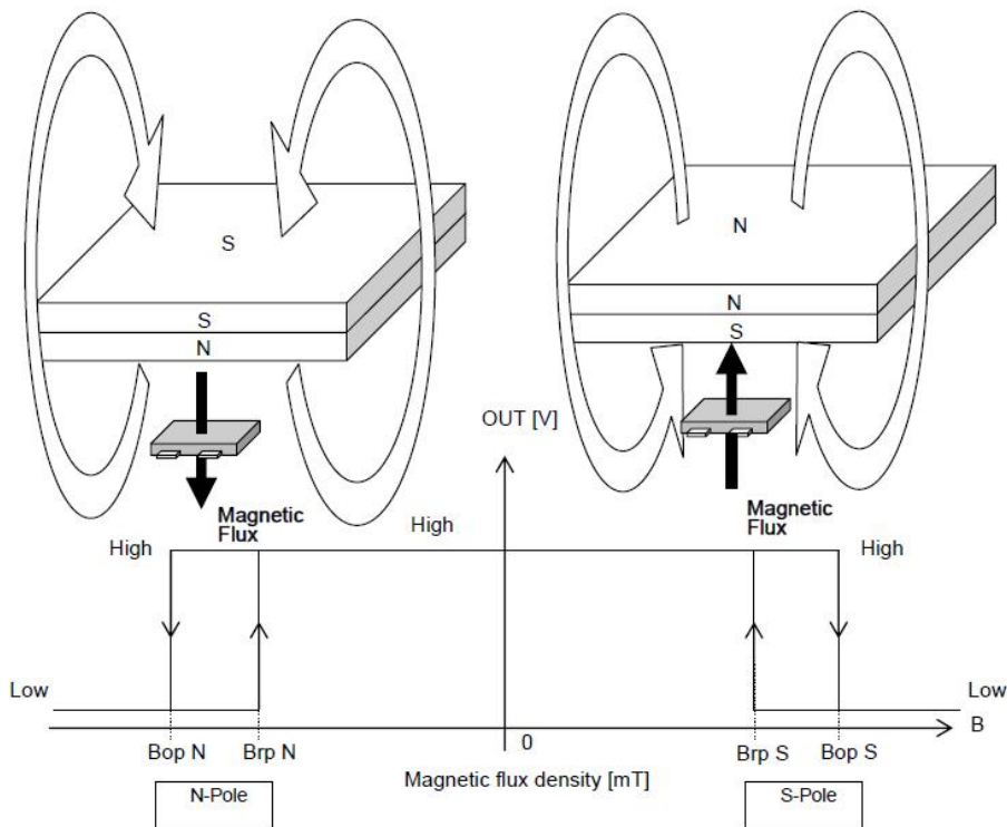
Fig 3, Magnetic Operation Characteristic of AS1832
